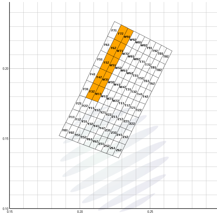
Fig. 1-6 The C.I.E Chromaticity Diagram CIE色度图
