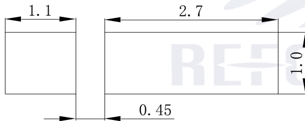
Fig.1-5 Soldering patterns 推荐焊盘
