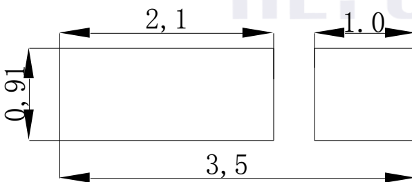
Fig.1-5 Soldering Patterns 推荐焊盘
